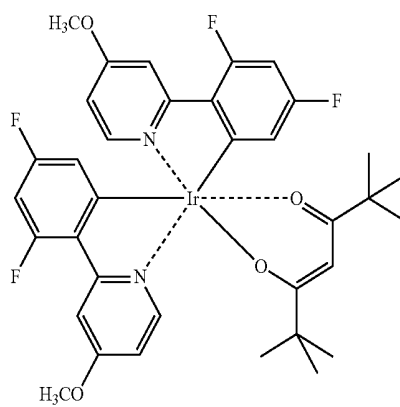
(F2ppy)2Ir(tmd)
