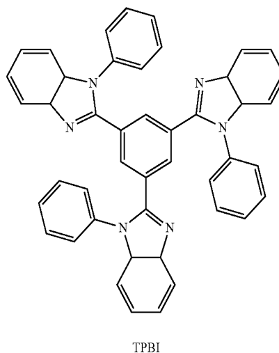
TPBI
