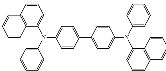
NPB
